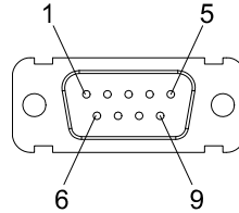
Figure 21: RS232 connector, male panel plug (front view)
