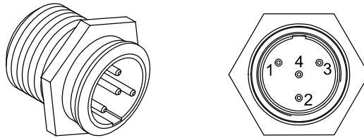
Figure 11: Male panel plug cod. TB4M (front view)
